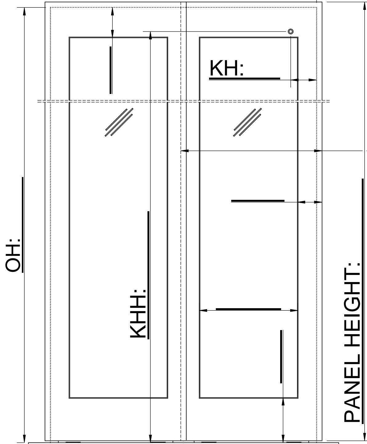
HALLSIDE ELEVATION (VIEW FROM HALLWAY)
